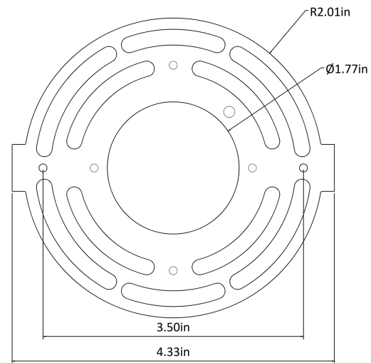
Drilling Pattern for Surface Mount
