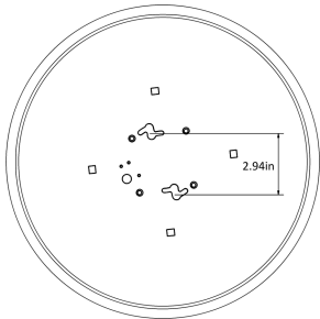
Screw Position for Surface Mount
