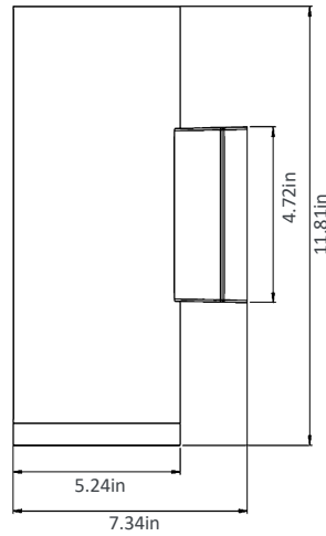
-WM-00 Wall Wall-mounted bracket
