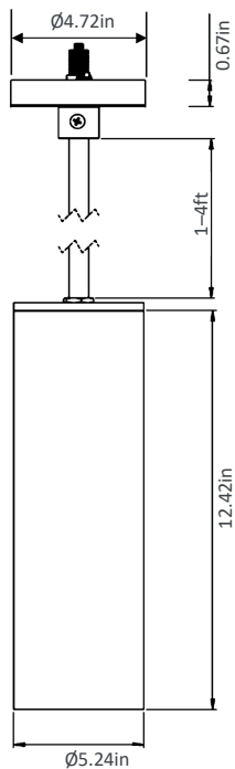
-SM-01 ... -SM-04 Stem Stem 0.5in thickness; 1ft, 2ft, 3ft & 4ft
