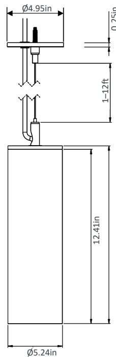
-PC-12 Pendant Aircraft cable, adjustable 1ft to 12ft
