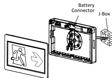
Wall mounting
