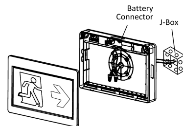
Wall mounting
