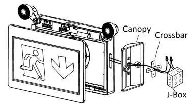
Side mounting
