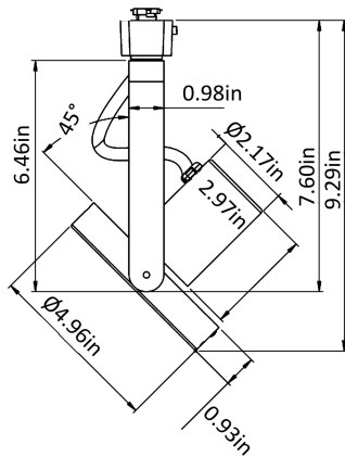
GBP38 Rear relamping gimbal
