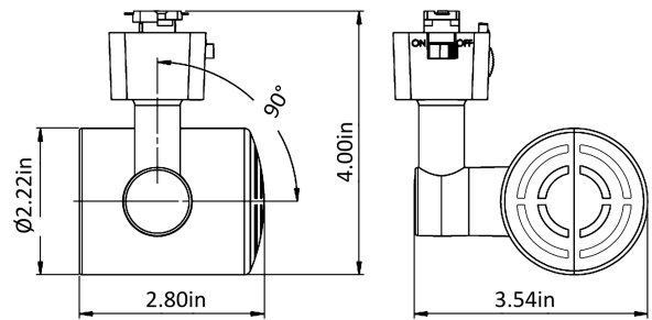
OLP00 Universal lamp holder
