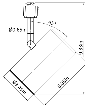
FCP20 Flat back cylinder
