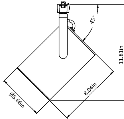
FCP38 Flat back cylinder
