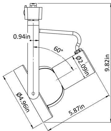
GFP38 Front relamping gimbal
