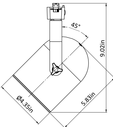
CLP30 Round back cylinder
