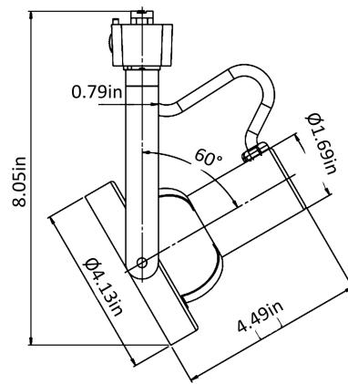
GFP30 Front relamping gimbal
