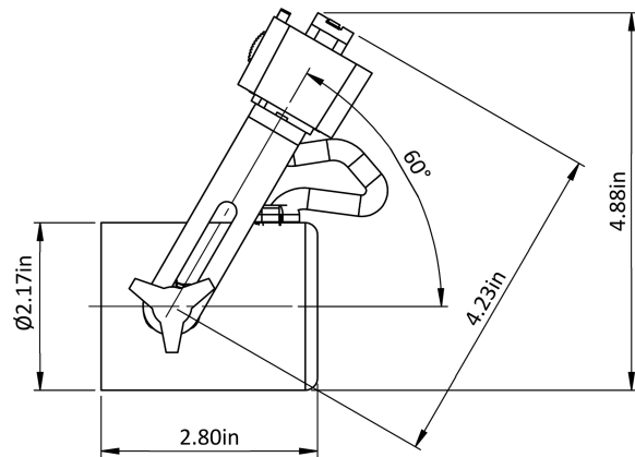
AJP00 Universal lamp holder
