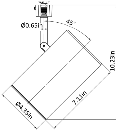
FCP30 Flat back cylinder
