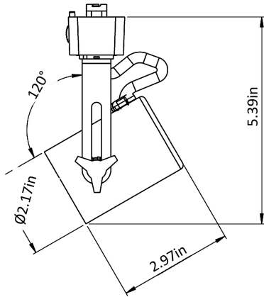
OOP00 Universal lamp holder, short neck
