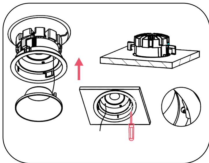
⑥ Insert housing to ceiling cut-out and tighten screws to lock the roto-lock mounting clips into place.
