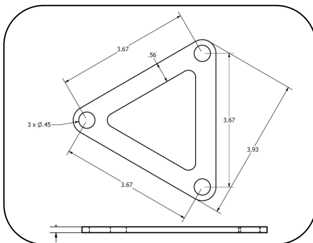
Dimensions of Anchor Bolt Carrier
