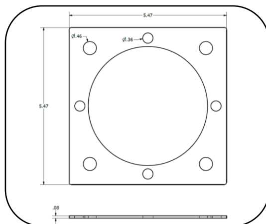
Anchor bolt carrier dimensions.
