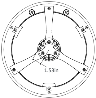
Pole Adapter
