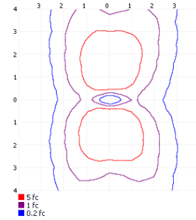
ISO footcandle plot
