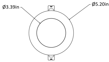
-4-15W Plan
