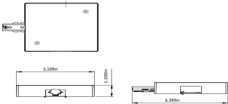
H10021 Single circuit end feed
