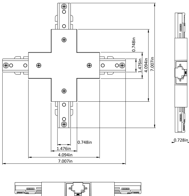
H10004 X connector
