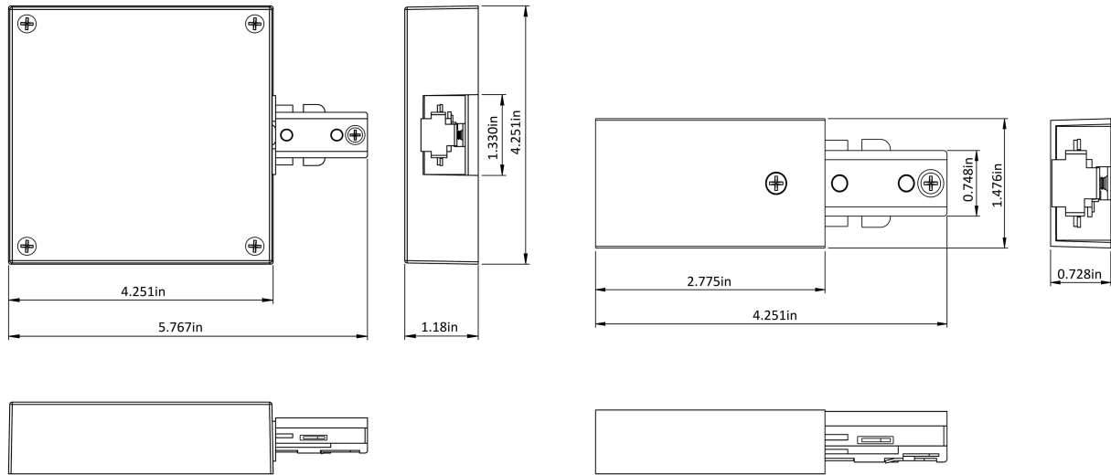
H10013 T-bar end feed
