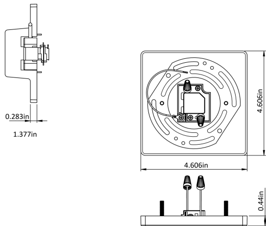
H10016 Monopoint adapter
