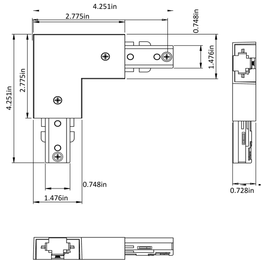
H10003 L connector
