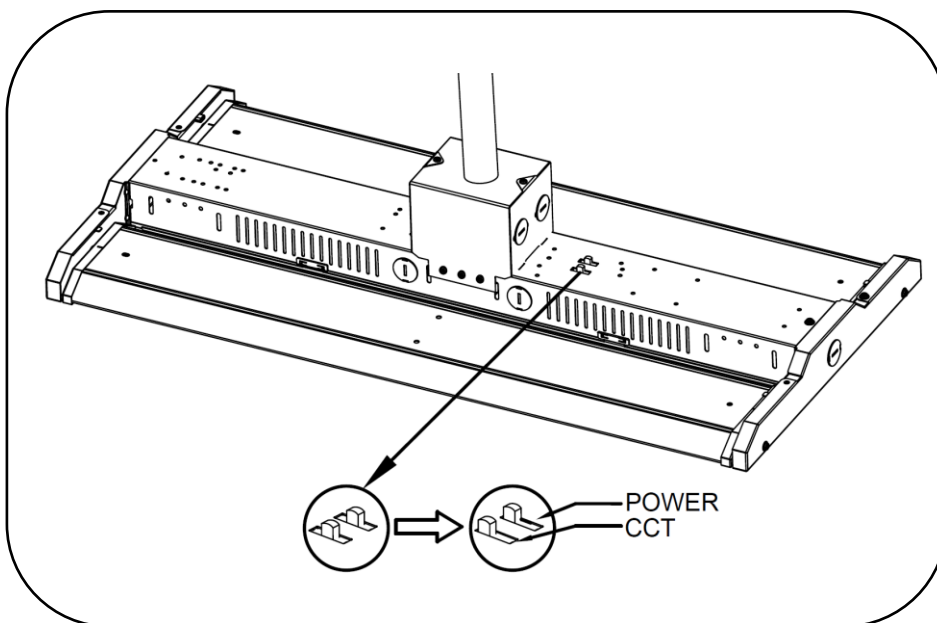
⑥ CCT/Power Changing.
