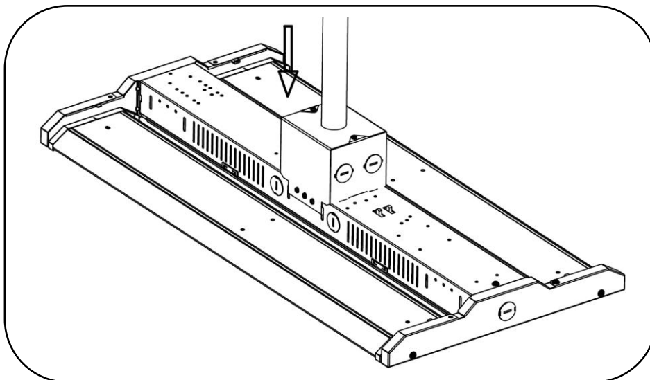
⑤ Pole Mounting installed.
