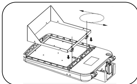
4x Short screws
